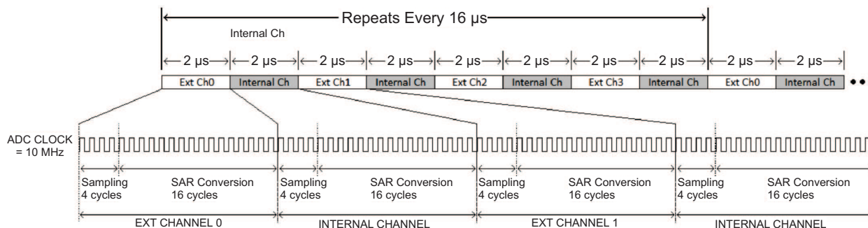
Figure 4-20. ADC Clock Timing Diagram
