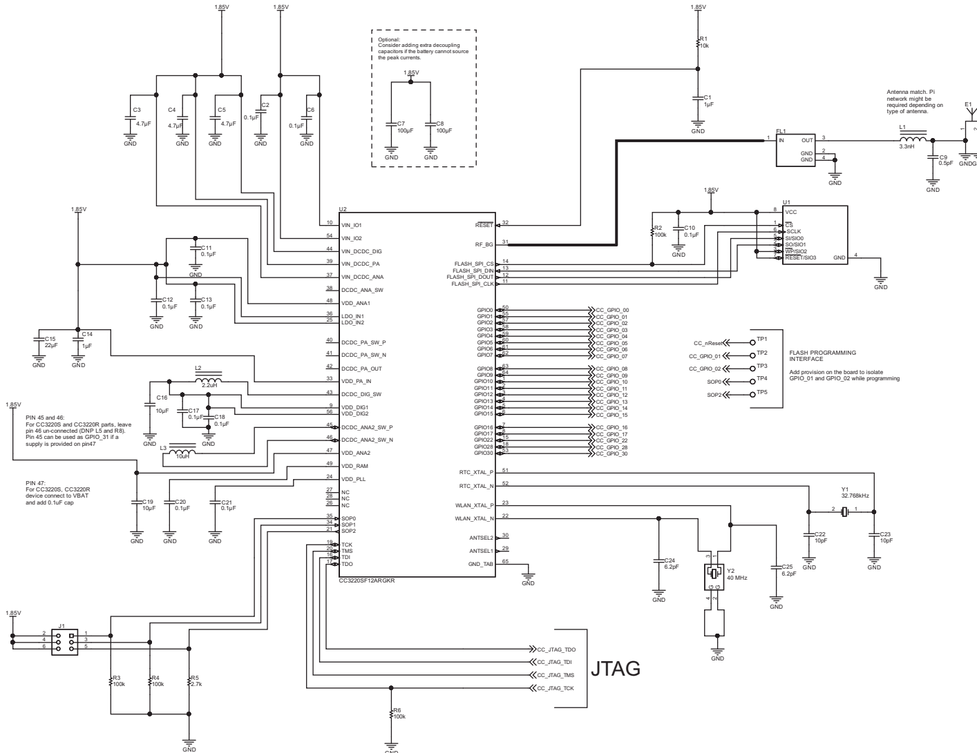
Figure 6-2. CC3220x Preregulated 1.85-V Mode Application Circuit
